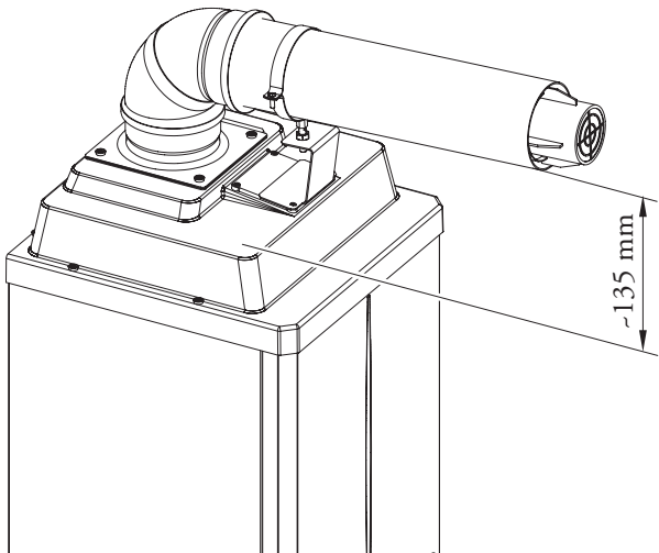
Horizontal concentric kit 80/125 - 3.025422 (required for external installation)
